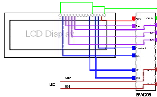
Figure 2 Minimal Wiring
